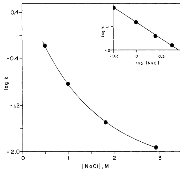
Figure 3. Effect of NaCl concentration on the thermal inactivation of glucose dehydrogenase at 85 °C. The first-order rate constants, k , of thermal inactivation were obtained from Figure 2.
